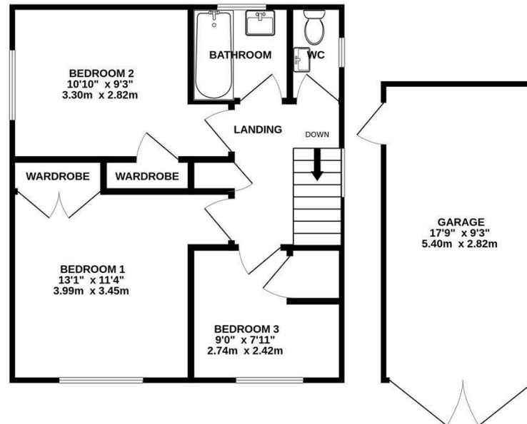
TOTAL FLOOR AREA : 1118 sq.ft. (103.9 sq.m.) approx.
